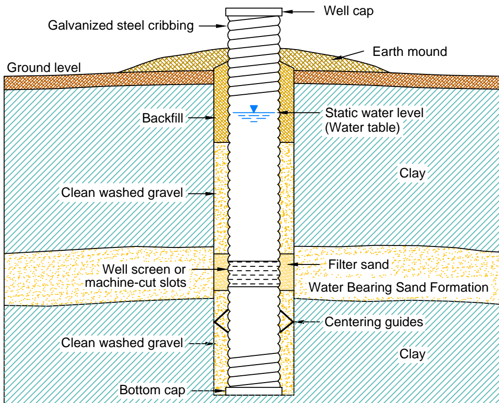
WELL CONSTRUCTION IN SHALLOW CONFINED AQUIFER
