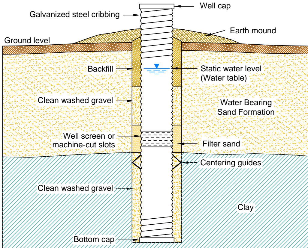
WELL CONSTRUCTION IN SHALLOW UNCONFINED AQUIFER
